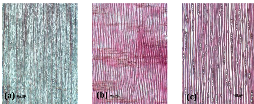
Gambar 3. Struktur mikro kayu agathis ( A. hamii ): penampang melintang, perbesaran 25x (a); penampang radial, perbesaran 50x (b) dan penampang tangensial, perbesaran 50x (c) Figure 3 Wood micro structure of agathis ( A. hamii ): transversal surface, magnification 25x (a); radial surface, magnification 50x (b) and tangential surface, magnification 50x (c)
